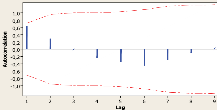
Autocorrelation Function for ISTIHDAM (with 5% significance limits for the autocorrelations)
