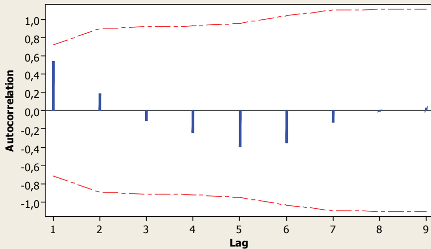
Autocorrelation Function for YATIRIM (with 5% significance limits for the autocorrelations)
